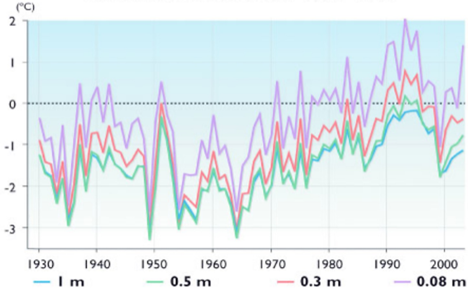
Average Annual Ground Temperature Fairbanks, Bonanza Creek 1930-2003
